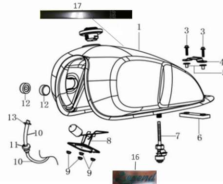
LEG150S-22 (FUEL TANK)
