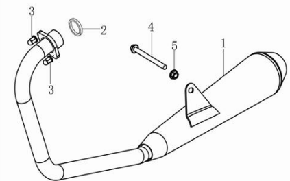
LEG150S-26 (MUFFLER ASSY)
