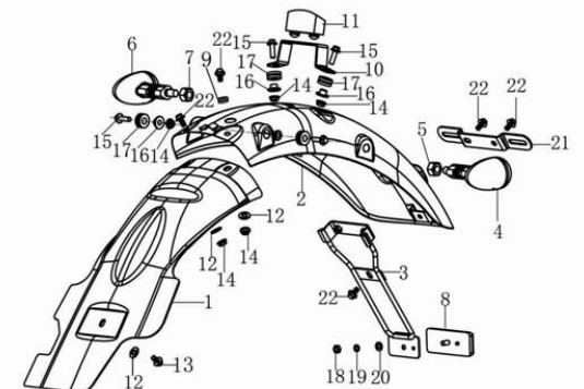
LEG150S-32 (TAIL LIGHT)
