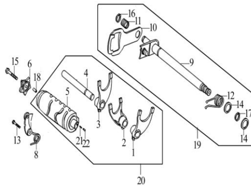
LEG150S-08 (SPEED CONTROL MECH.)
