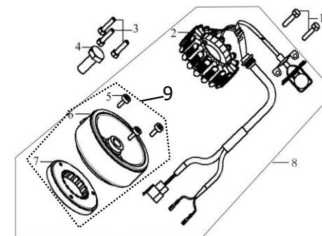
LEG150S-12 (GENERATOR ASSY.)
