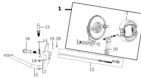
LEG150S-31 (REAR BREAK ASSY)
