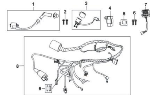
LEG150S-35 (ELECTRICAL PARTS)
