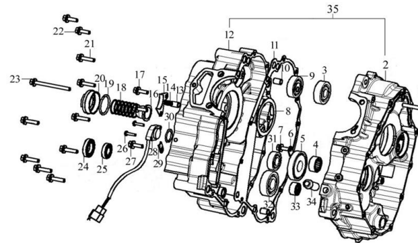
LEG150S-08 (SPEED CONTROL MECH.)
