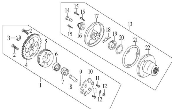
LEG150S-13 (LH. CRANKCASE COVER)
