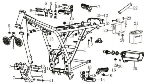
LEG150S-33 (FRAME & FOOTREST)
