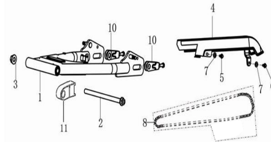
LEG150S-25 (SWING ARM & CHAIN BOX)
