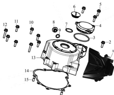
LEG150S-13 (LH. CRANKCASE COVER)
