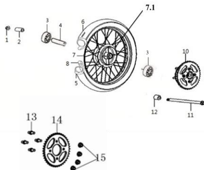
LEG150S-30 (REAR WHEEL)
