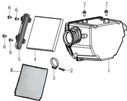
LEG150S-36 (AIR FILTER)
