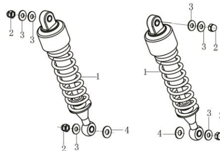
LEG150S-28 (REAR SHOCK)
