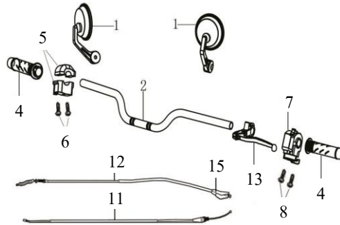
LEG150S-16 (HANDLE BAR & REAR MIRROR)
