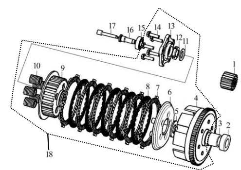
LEG150S-09 (CLUTCH ASSY.)
