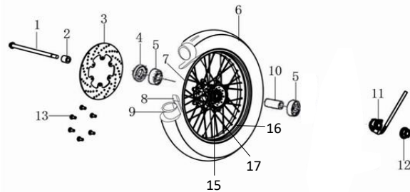
LEG150S-21 (FRONT WHEEL ASSY)
