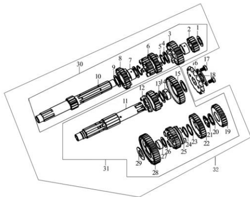
LEG150S-07 (ACTUATING MECH. ASSY.)
