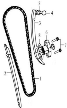
LEG150S-07 (ACTUATING MECH. ASSY.)
